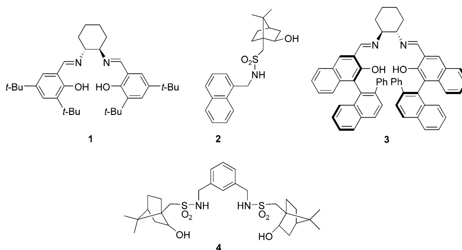
Scheme 1. Various efficient ligands for the asymmetric alkynylation of aliphatic ketones.
