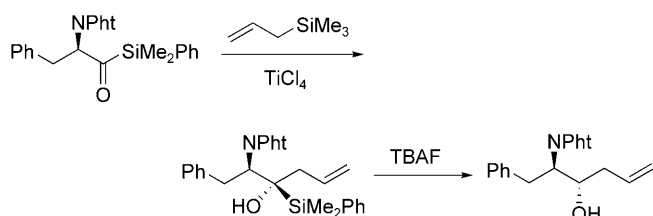
Scheme 2. Acylsilane as stable synthetic equivalent of \alpha -amino aldehyde.
